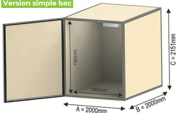
Version simple bac
